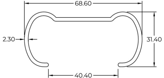
Side Rail 5354D WT : 0.818 KG/M
