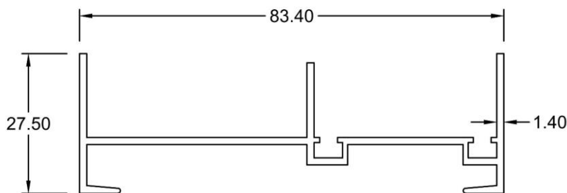
2-Track Outer Vertical 17205 WT : 0.682 KG/M
