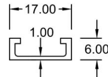
Bottom Track (Showcase U) 5101 WT : 0.100 KG/M
