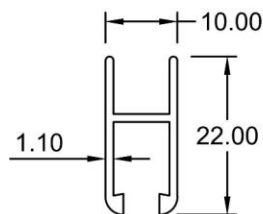
Inner Bottom (Showcase H) 5100 WT : 0.168 KG/M
