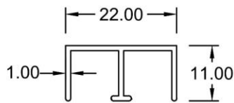
Top (Showcase) 5300 WT : 0.148 KG/M
