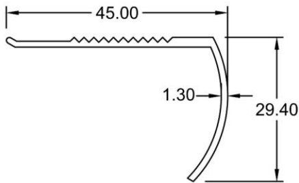
Stair Nosing 1885
