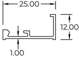
Glazing Bead SPF5
