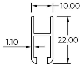
Inner Bottom (Showcase H) 5100
