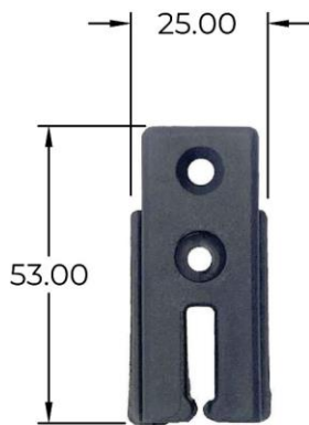
Inner Top Guide HDB-442 for window / door
