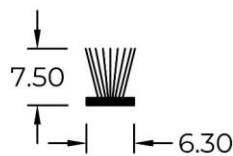
WP-63-750-3P
