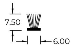
WP-60-750-3P
