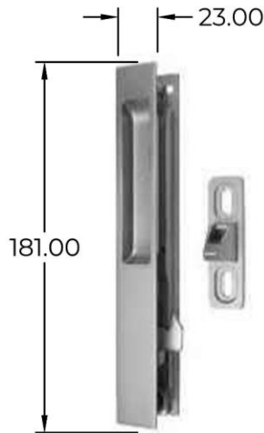
Door Lock LK-A5-NA without key
